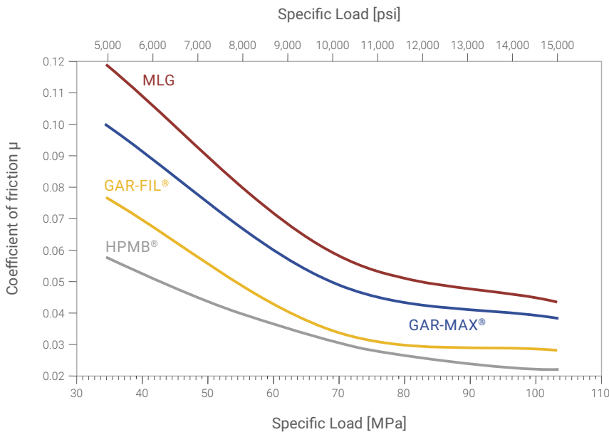
Fig.5: Coefficient of friction vs specific load
